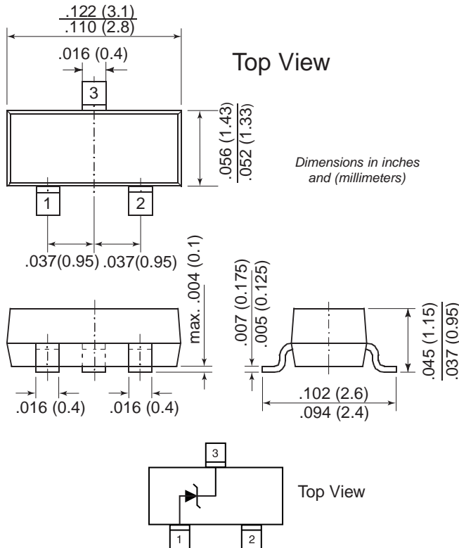
TO-236AB (SOT-23)
